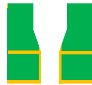
Back Drill Via Accuracy range : \pm 50 \mu m
