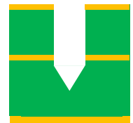
Blind Via Accuracy range: \pm 12 \mu m
